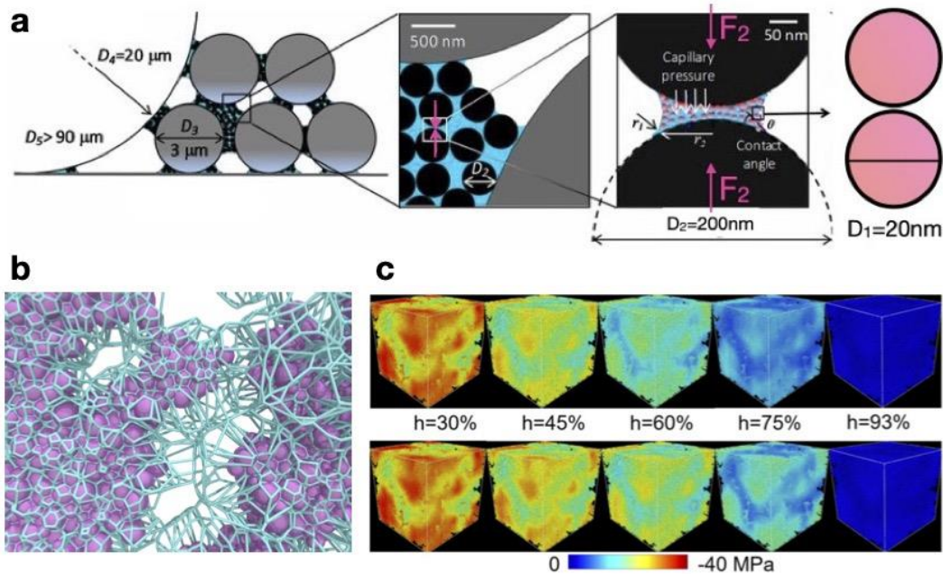
Figure. a) Formation of solid bridges induced by capillary forces at the nanoscale stabilize polydisperse size aggregates at the macroscale [1]. b) Computation of capillary forces using voronoi tessellation [2]. c) Local variation of capillary pressure of a porous sample of cement with increasing/decreasing relative humidity [3].
